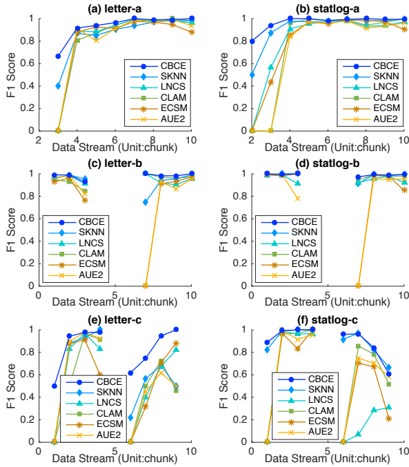
Fig. 7. F1 scores on the synthetic streams.
