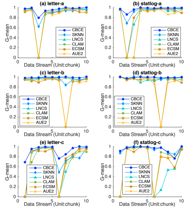
Fig. 8. G-means on the synthetic streams.
