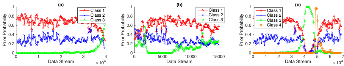
Fig. 4. Three class evolution scenarios of the comparative study on tweet data.
