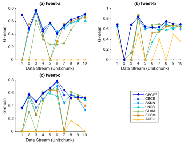
Fig. 10. G-means on the tweet streams.
