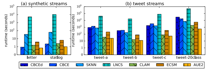
Fig. 11. Runtime of the compared approaches.
